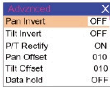
Figure 6-5 Advanced setting
