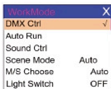
Figure 6-2 Run Settings
