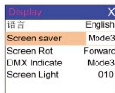
Figure 6-3 Display Settings
