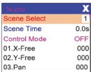
Figure 6-4 Scene Settings
