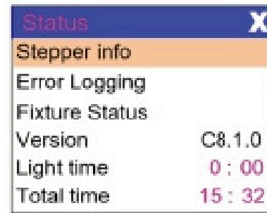
Figure 6-6 Status Settings
